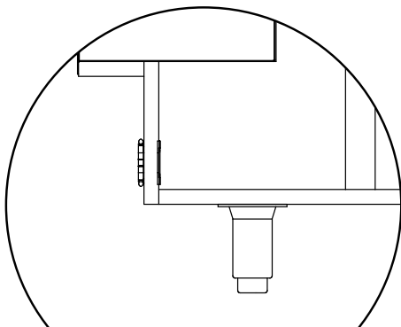
Adjustable Foot
